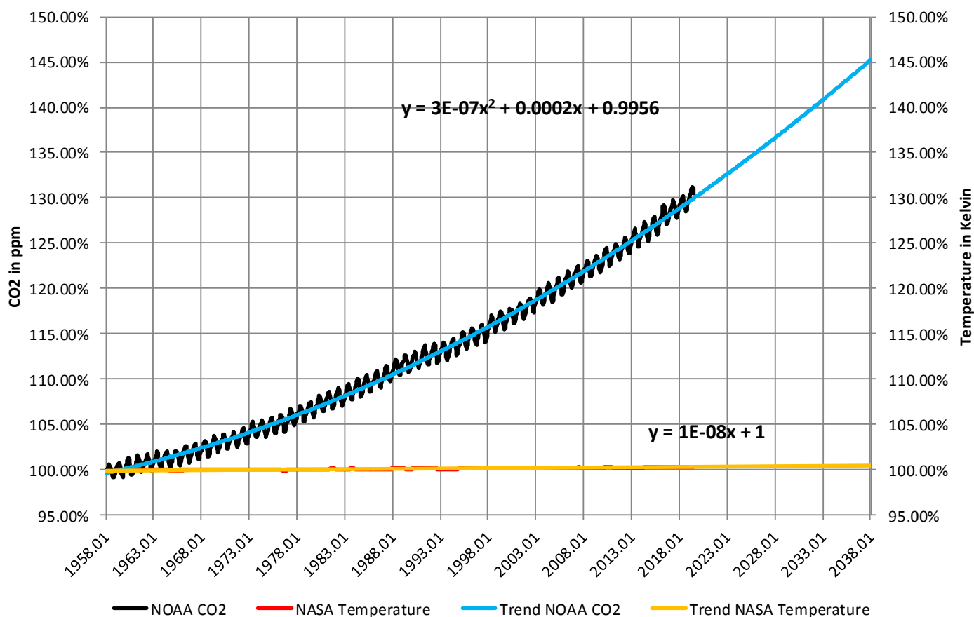
Chart 8a, CO 2 and Temperature % Change from 1958
