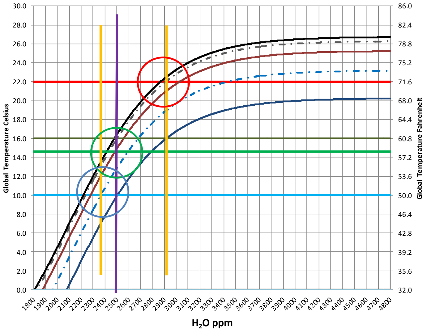
Chart 13, Global Temperature H 2 O + CO 2 Logistics Function
