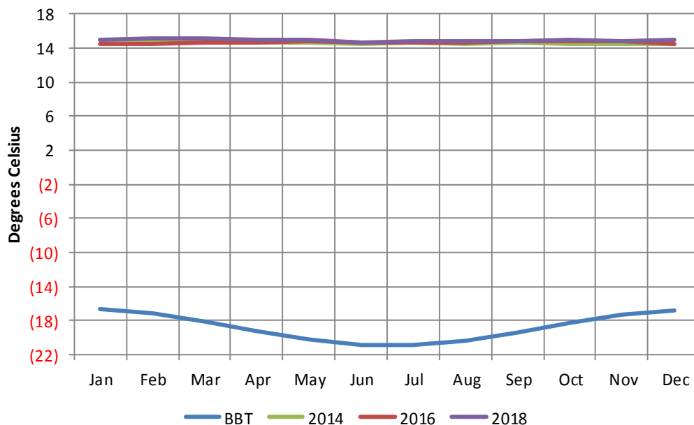
Chart 17, Black Body Temperature Verses Monthly LOTI Values
