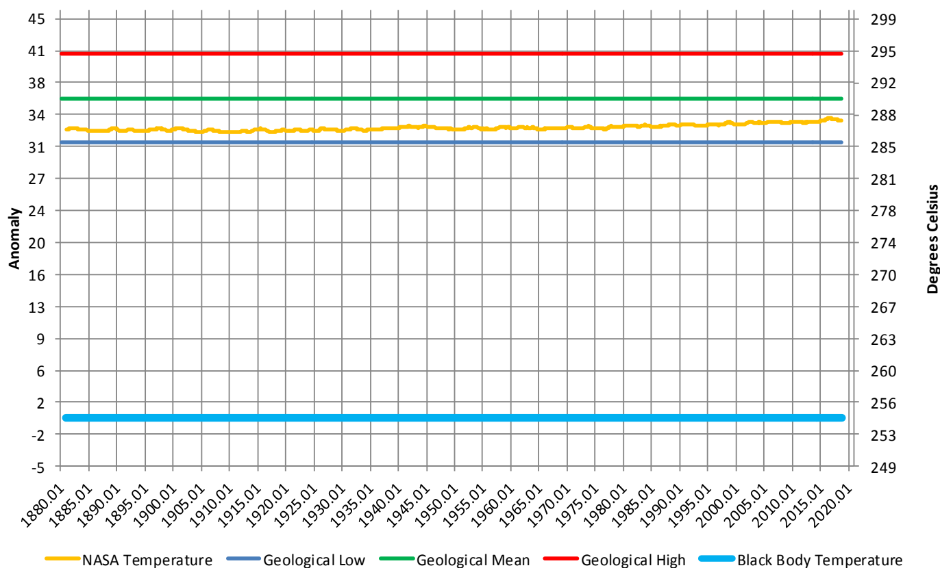
Chart 15, NASA Anomalies using the Planets Black Body Temperature of 254.36 degrees as the base.
