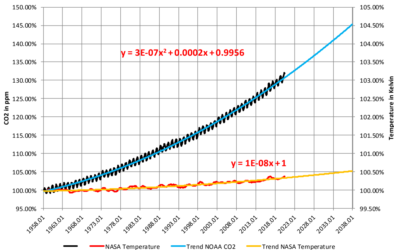
Chart 8, CO2 and Temperature % Change from 1958
