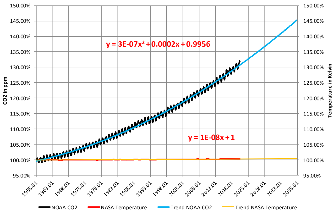
Chart 8a, CO2 and Temperature % Change from 1958
