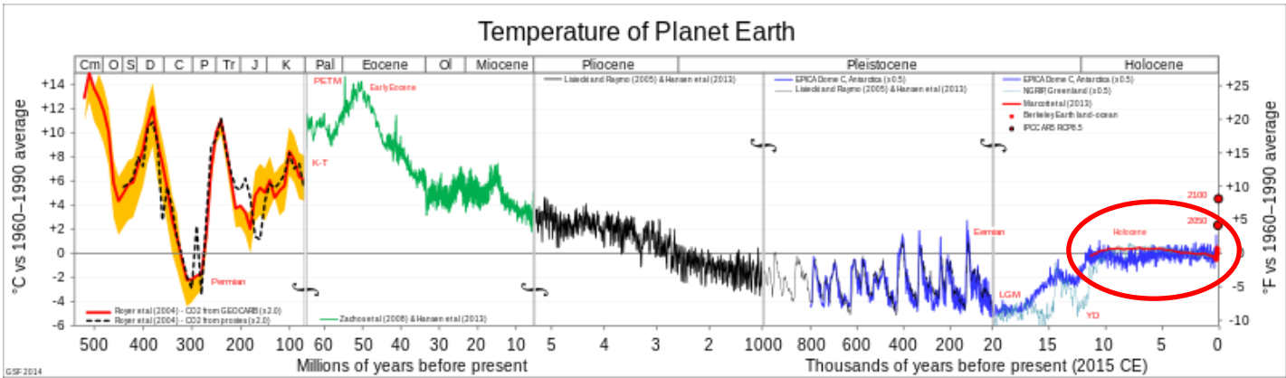
Figure 8, NASA Official Temperatures
