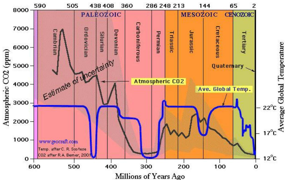
Figure 4, Geological temperatures and Carbon Dioxide
