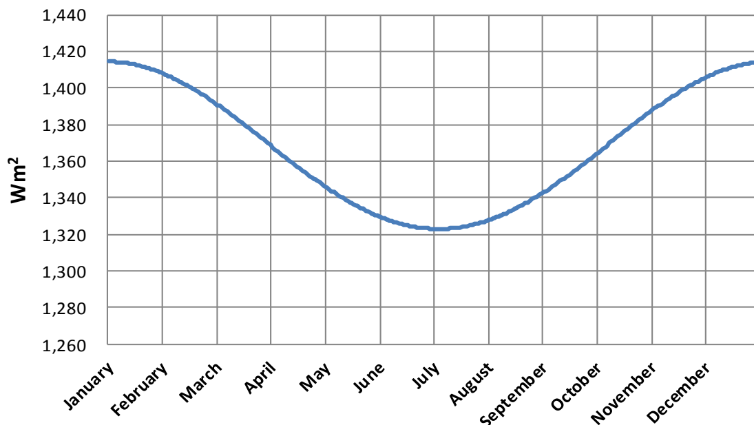
Chart 13, Solar Flux Earth
