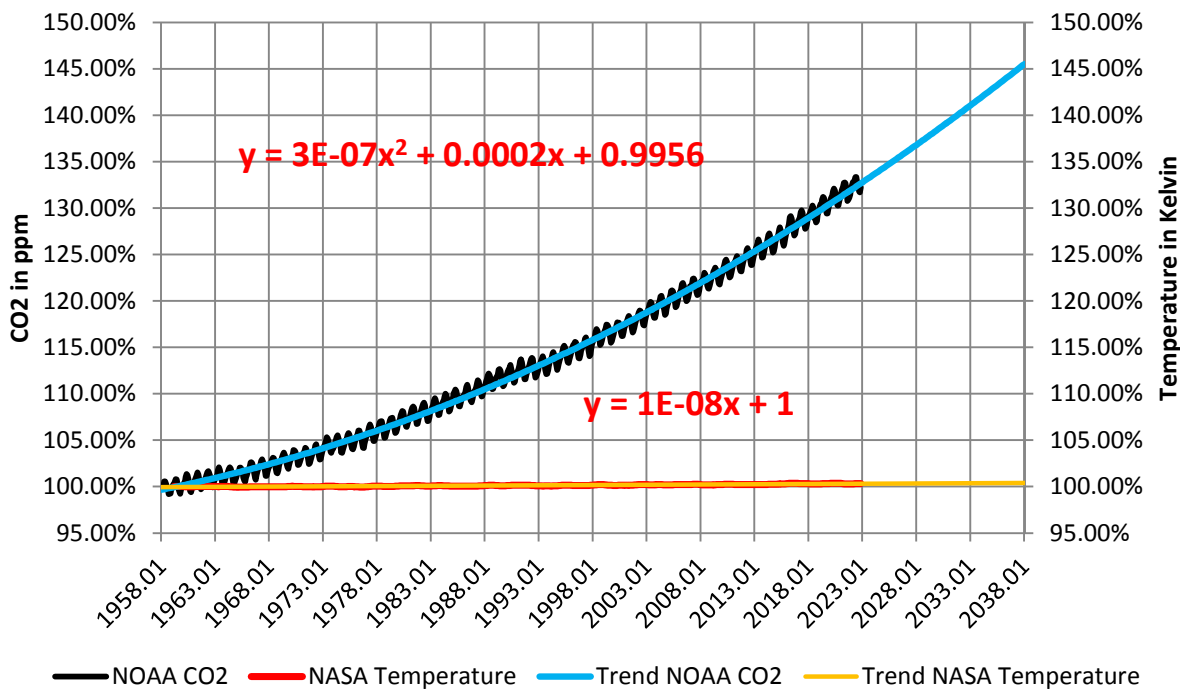
Chart 8a, CO 2 and Temperature % Change from 1958
