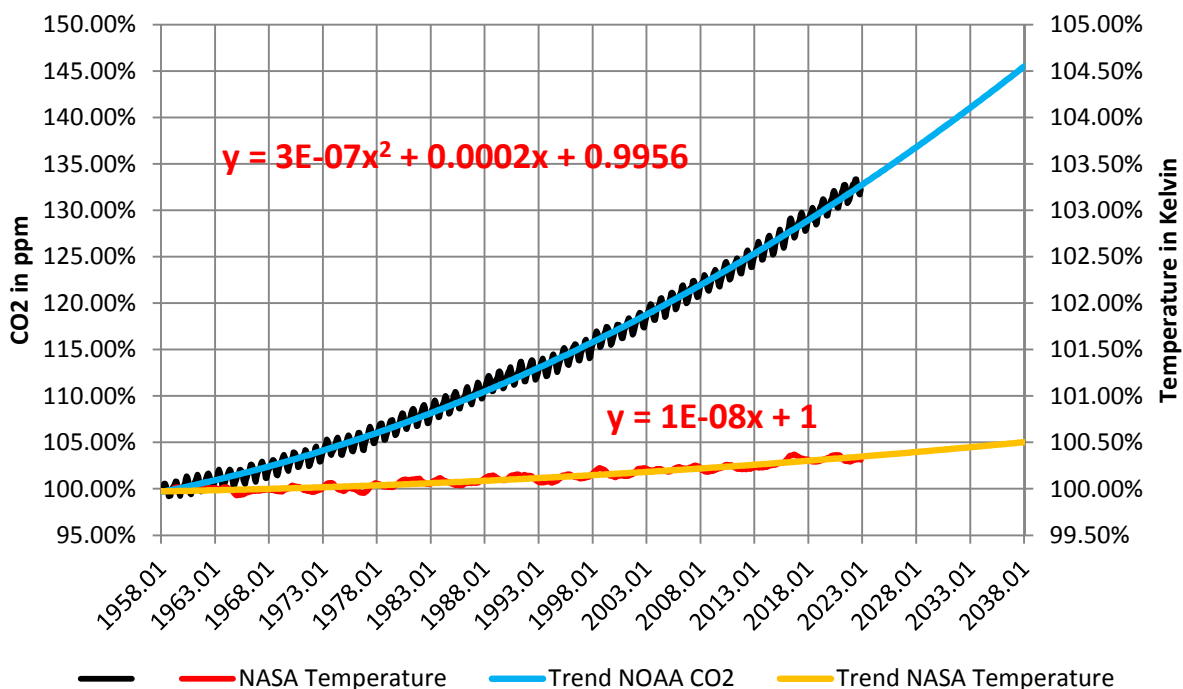
Chart 8, CO2 and Temperature % Change from 1958
