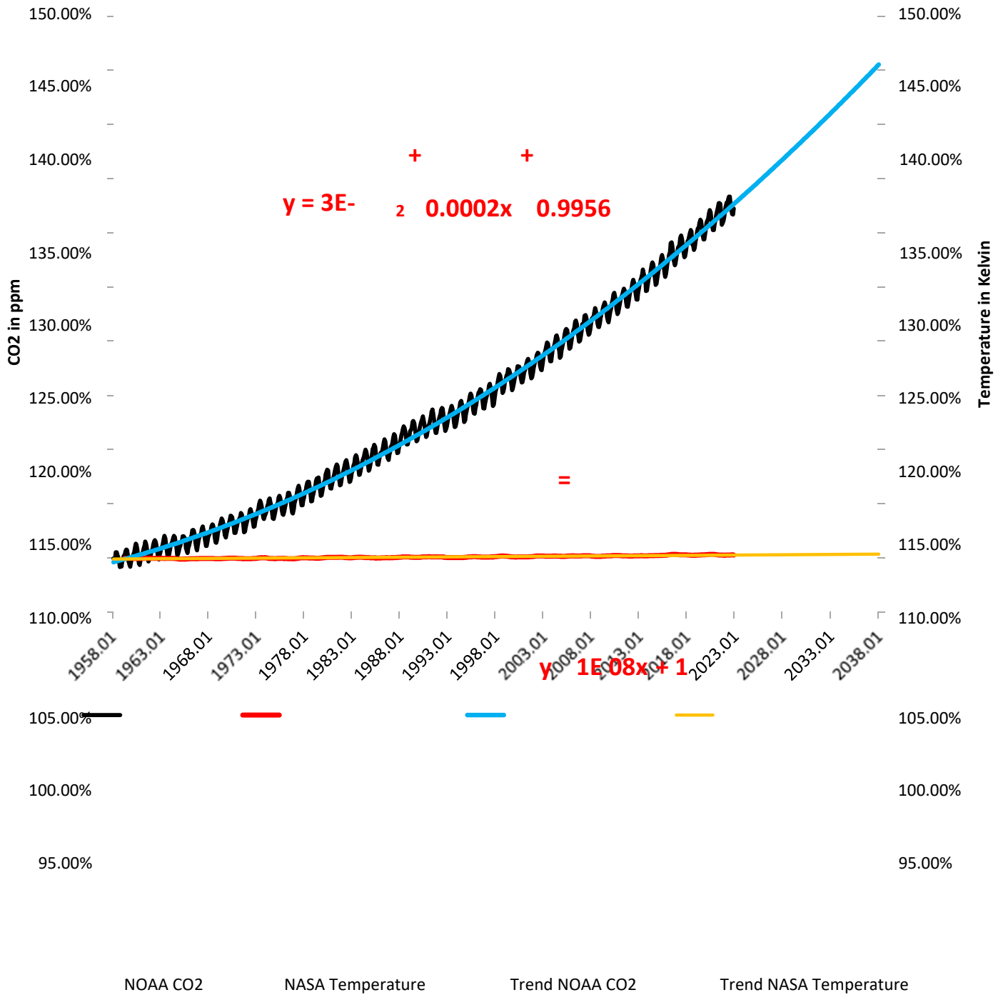
Chart 8a, CO2 and Temperature % Change from 1958
