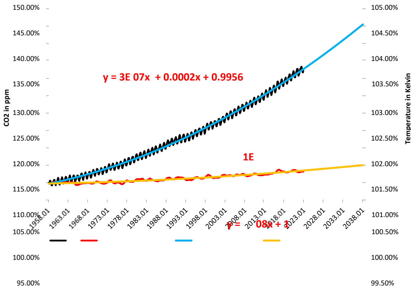
Chart 8, CO 2 and Temperature % Change from 1958
