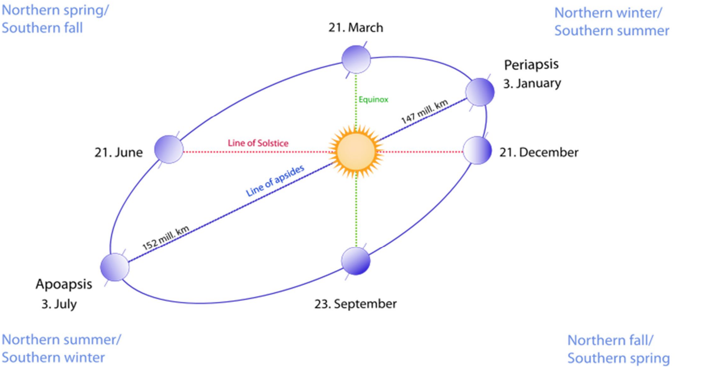
Figure 1, the Earth’s orbit
